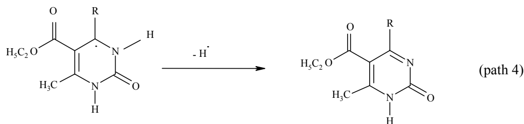
Scheme 3. Proposed mechanism for dehydrogenation of DHPMs by \text{K}_2\text{S}_2\text{O}_8
