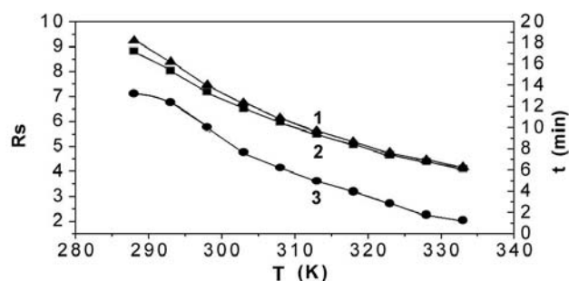
Fig. 5. Effect of temperature on R_s and migration time: 1) t_{S\text{-clenbuterol}} ; 2) t_{R\text{-clenbuterol}} ; 3) R_s . Conditions: as given in Fig. 2.
