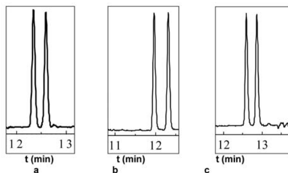
Fig. 1. Effect of chiral selector on the enantioseparation of clenbuterol. Conditions: 60/50 cm × 50 μm i.d. fused-silica capillary, 24 kV, 20 °C, λ = 214 nm; 50 mmol l -1 H 3 PO 4 /H 2 PO 4 - buffer (pH 2.5); injection: 20 psi during 5 s; (a) 10 mmol l -1 β-CD; (b) 10 mmol l -1 HP-β-CD; (c) 10 mmol l -1 DM-β-CD.
