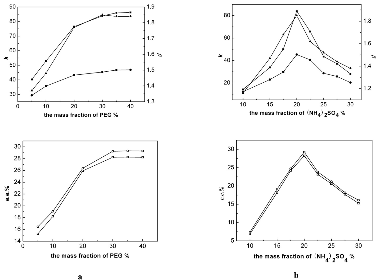
Fig. 3. Influence of the mass fraction of PEG and (NH_4)_2SO_4 . a) Influence of the mass fraction of PEG on the distribution behavior of MA enantiomer. D,L -MA 0.11 M, \beta -CD 0.004 M, the mass fraction of (NH_4)_2SO_4 is 20%, the polymerization degree of PEG is 2000, pH 1.0 and temperature: 30 °C; b) Influence of the mass fraction of (NH_4)_2SO_4 on the distribution behavior of MA enantiomer. D,L -MA 0.11 M, \beta -CD 0.004 M, the mass fraction of PEG is 30%, the polymerization degree of PEG is 2000, pH 1.0 and temperature: 30 °C. (■) K_D , (●) K_L , (▲) \beta , (□) the bottom phase, (○) the top phase).
