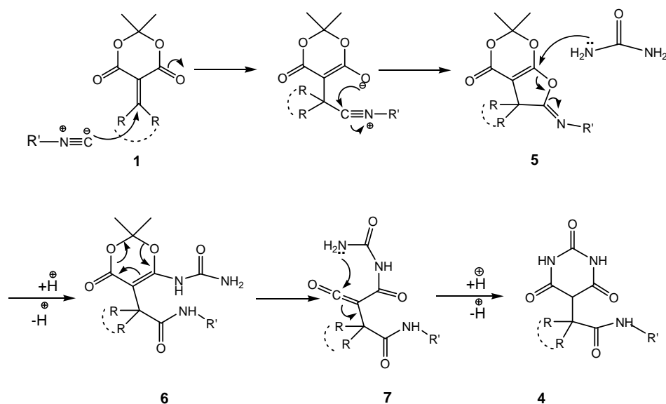
Scheme 2. Proposed mechanism for the reaction
