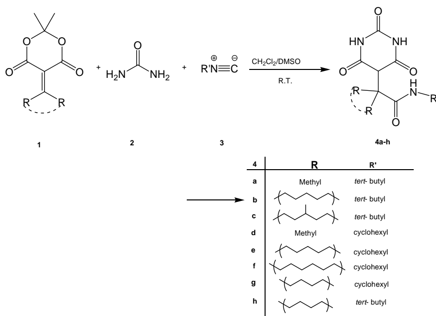
Scheme 1. Multi-component reaction of alkylidene Meldrum's acid, alkyl isocyanide and urea
