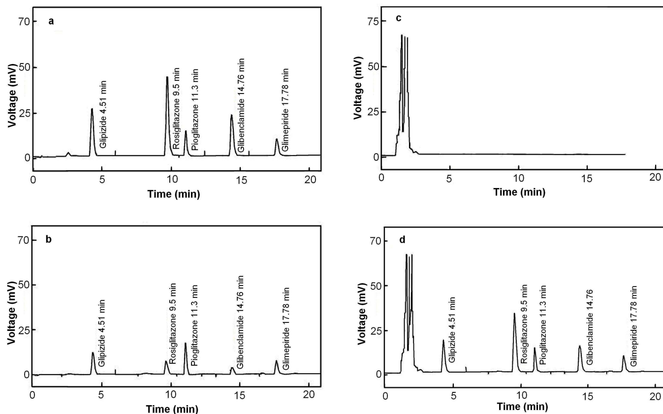
Fig. 2. Chromatograms showing the retention times of Glipizide, Rosiglitazone, Pioglitazone, Glibenclamide and Glimepiride at a concentration of 20 \mu\text{g ml}^{-1} in Pure (a), formulation mixture (b) blank plasma (c) and Human Plasma (d).
