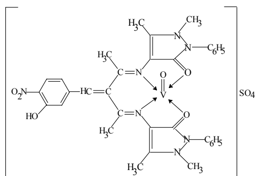
Fig. 2. The proposed structures of the Schiff base complexes.
