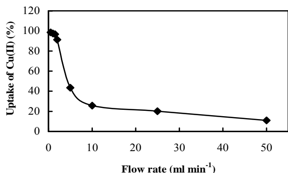
Fig. 4. Uptake (%) of \text{Cu}^{2+} ions by diamine-thiol polysiloxane immobilized ligand system (DTP) vs. flow rate in \text{ml min}^{-1} (bed material = 3 g, mesh size = 60-80, pH = 5.5).
