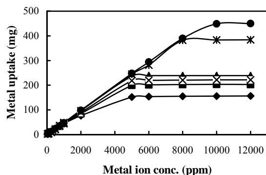
Fig. 3. Metal uptake by diamine-thiol polysiloxane immobilized ligand system (DTP) vs. concentration of metal ions using column method (bed material = 3 g, mesh size = 60-80, flow rate = 1.0-1.5 ml min -1 , pH = 5.5): (◆) Co(II), (■) Ni(II), (▲) Cu(II), (×) Zn(II), (★) Cd(II) and (●) Pb(II).
