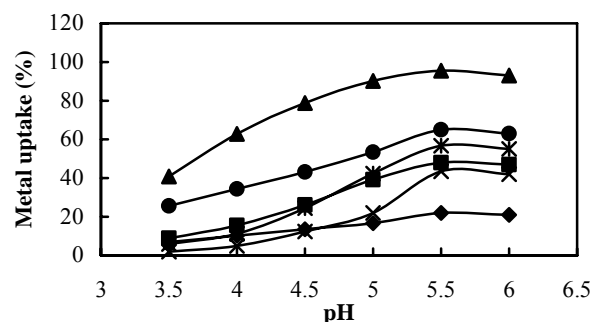
Fig. 2. Uptake (%) of metal ions by diamine-thiol polysiloxane immobilized ligand system (DTP) vs. pH using column method (bed material = 3 g, mesh size = 60-80, flow rate = 1.0-1.5 ml min -1 ): (◆) %Co(II), (■) %Ni(II), (▲) %Cu(II), (×) %Zn(II), (★) %Cd(II) and (●) %Pb(II).
