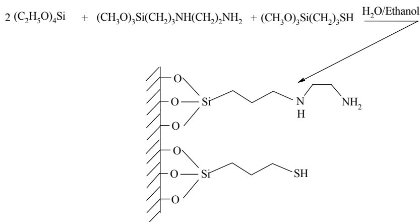
Scheme 1. Preparation of diamine-thiol polysiloxane ligand system (DTP)
