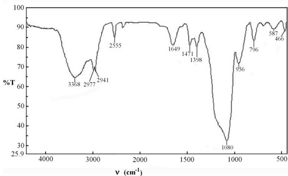
Fig. 1. FTIR spectrum of diamine-thiol polysiloxane immobilized ligand system (DTP).
