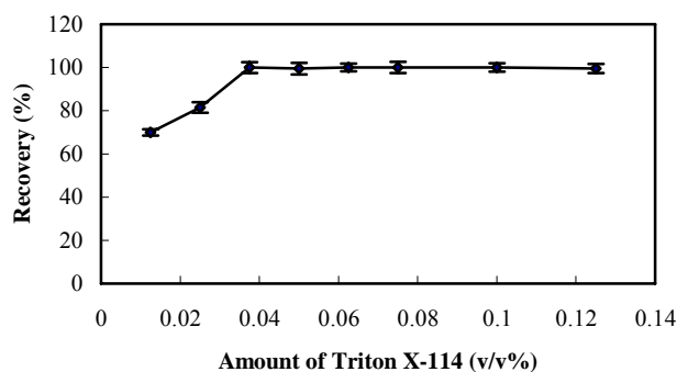
Fig. 4. Effect of Triton X-114 concentration on the CPE of iron. Conditions: iron concentration, 125 \mu\text{g l}^{-1} ; concentrated volume, 20 ml; ferron, 1.4 \times 10^{-4} M; pH \sim 5 ; TBT, 0.01 M.
