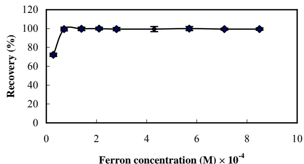
Fig. 3. Effect of ferron concentration on the CPE of iron. Conditions: iron concentration, 125 \mu\text{g l}^{-1} ; concentrated volume, 20 ml; Triton X-114, 0.05% (v/v); pH \sim 5 ; TBT, 0.01 M.
